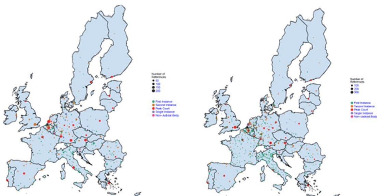
Figure 3 Left: 2004-2014 | Right: 1961-2014
